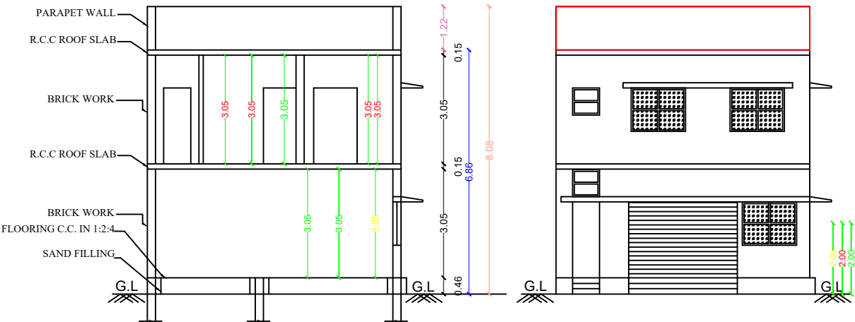
SECTION"A-B"
