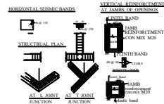
STRUCTURAL PLAN
