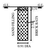
SECTION ON "A-B"
