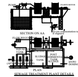
SECTION ON A-A
