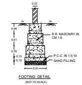
FOOTING DETAIL (NOT TO SCALE)
