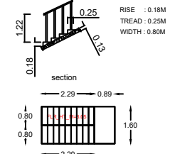
STAIRCASE DETAIL
