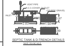
SEPTIC TANK & D-TRENCH DETAILS NOT TO SCALE
