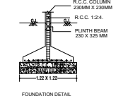
FOUNDATION DETAIL (NOT TO SCALE)
