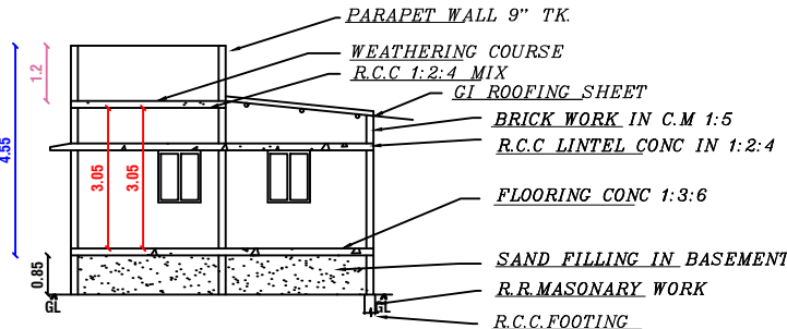
SIDE SECTION
