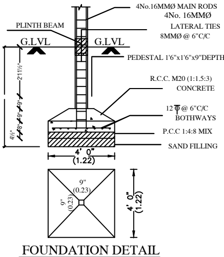
FOUNDATION DETAIL
