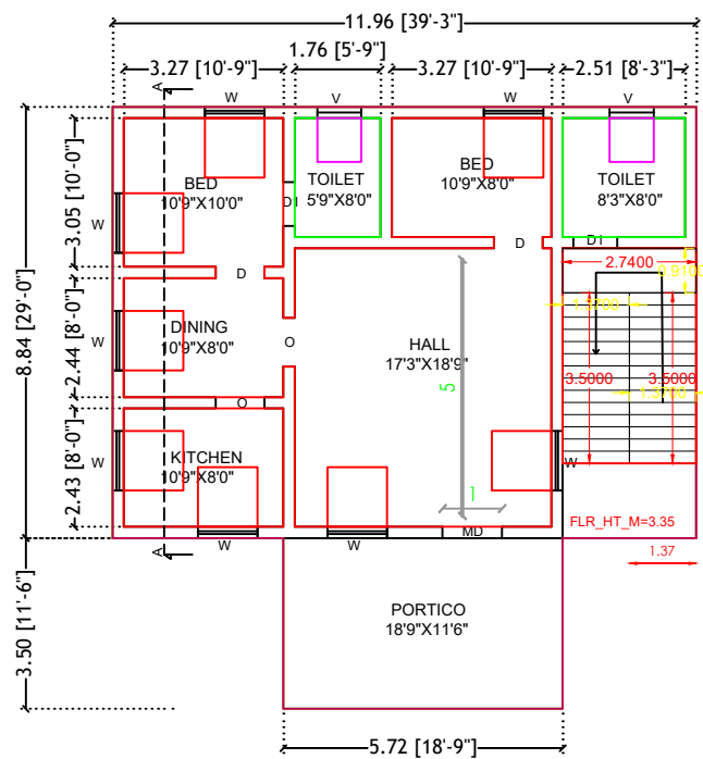
IND FLOOR PLAN
