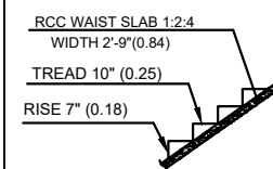
STAIRCASE DETAIL SCALE 1:50
