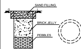
RAIN WATER HARVESTING SYSTEM SCALE 1:50
