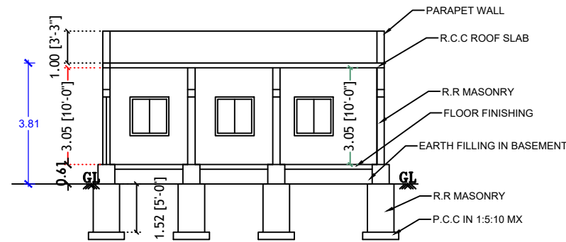
SECTION ON-AA
