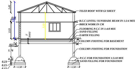
SECTION ON-AA
