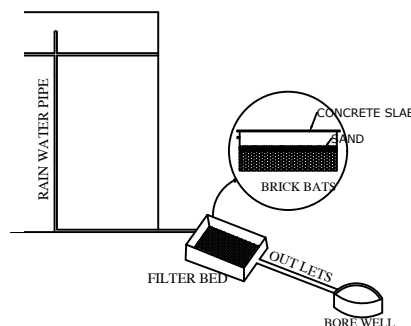
RAIN WATER HAVESTING TANK
