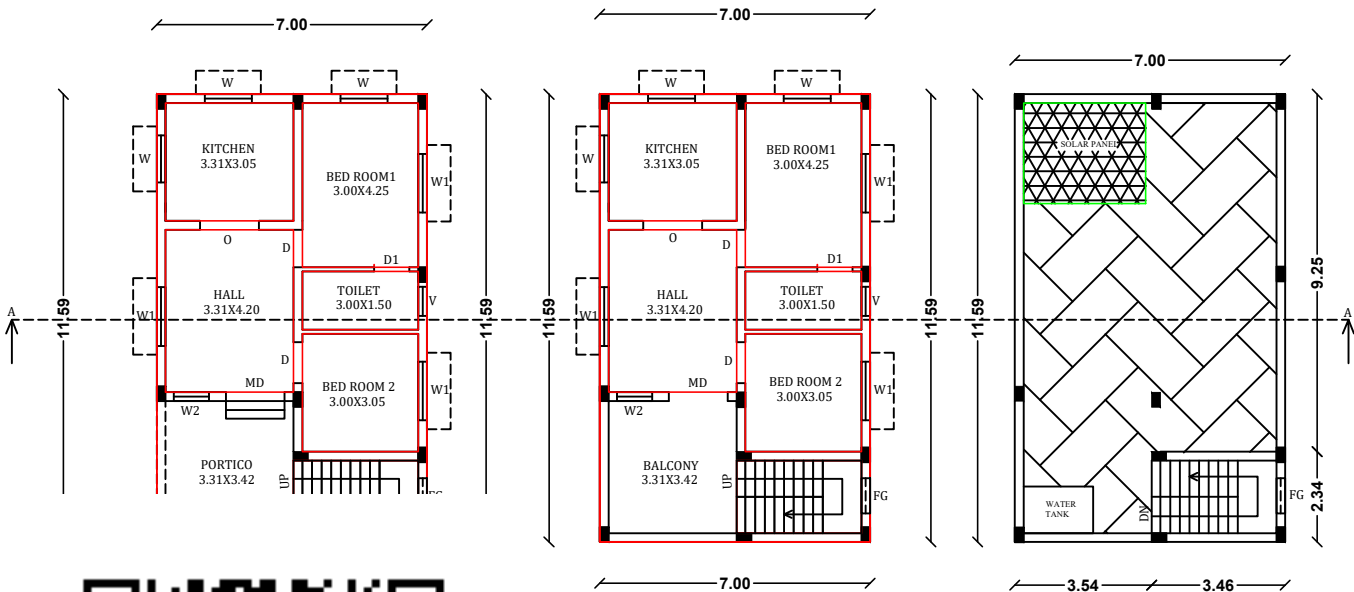
FLOOR- FIRST
