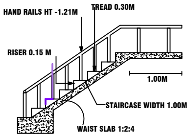
STAIRCASE DETAILS
