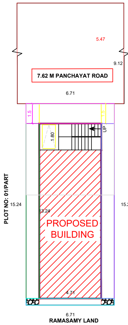
SITE PLAN:PROPOSED SCALE 1:100
