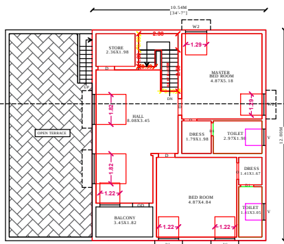
FLOOR - FIRST PRO. FIRST FLOOR PLAN
