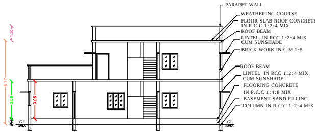
CROSS SECTION ON "A-A"
