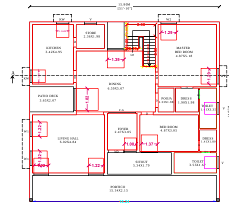
FLOOR - GROUND PRO. GROUND FLOOR PLAN
