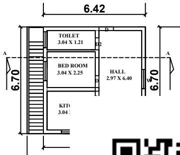
FLOOR- PRO.GR
