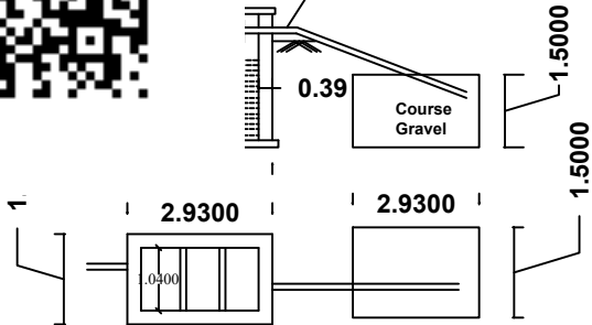
SEPTIC TANK & D-TRENCH DETAILS
