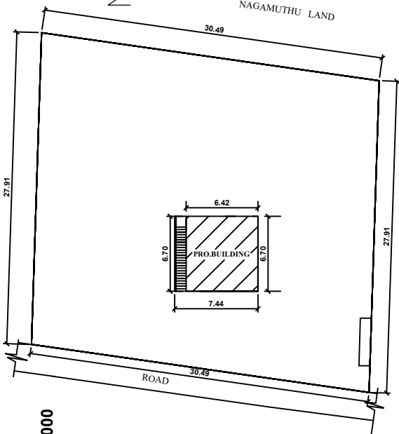
SITE PLAN
