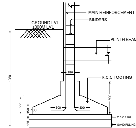
TYPICAL SECTION OF R.C.C COLUMN FOUNDATION SCALE : 1" = 2'-0"
