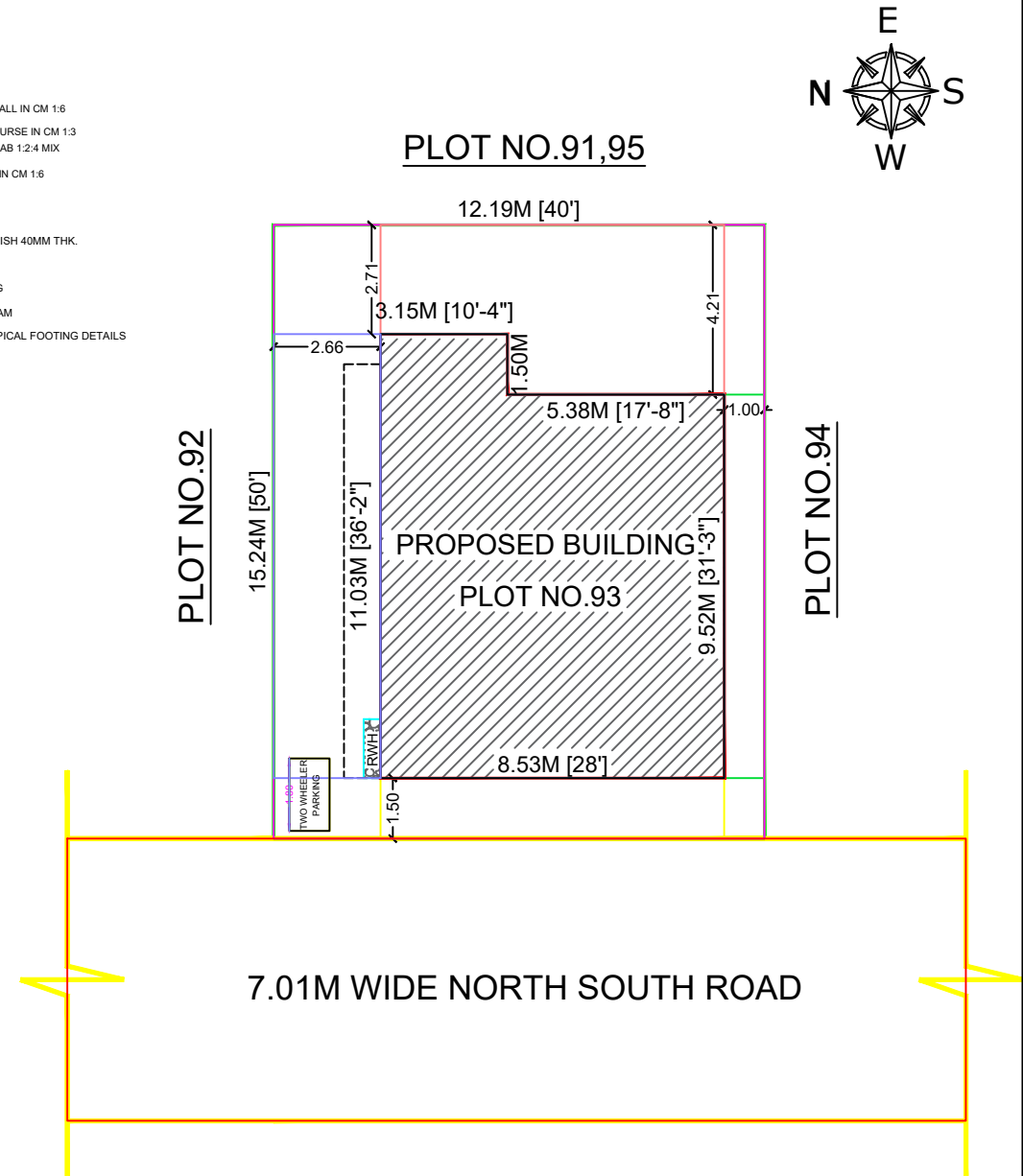
SITE PLAN
