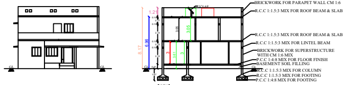
FRONT ELEVATION
