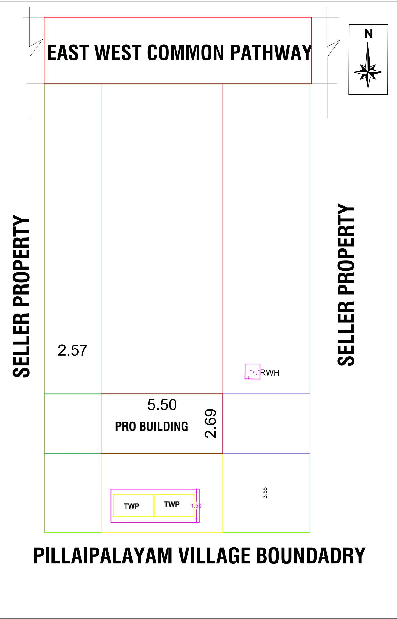
SITE PLAN
