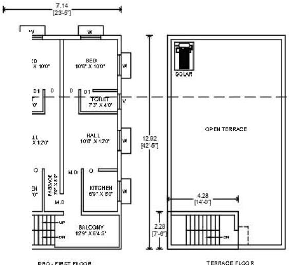
PRO - FIRST FLOOR
