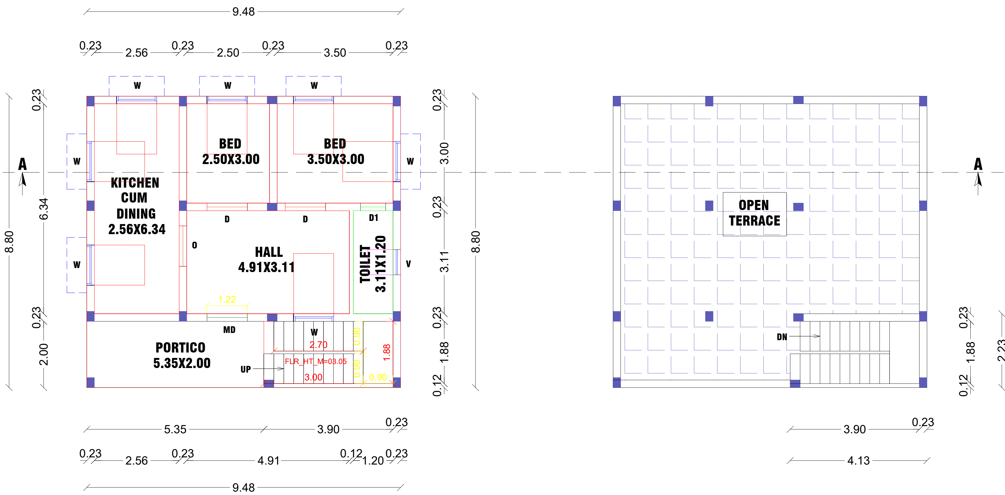
FLOOR-GROUND
