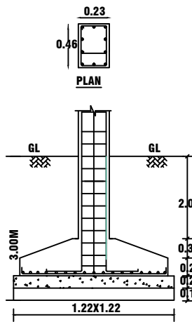
COLUMN DETAILS
