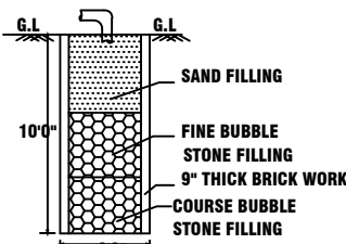
SECTION ON RAIN WATER COLLECTION TANK
