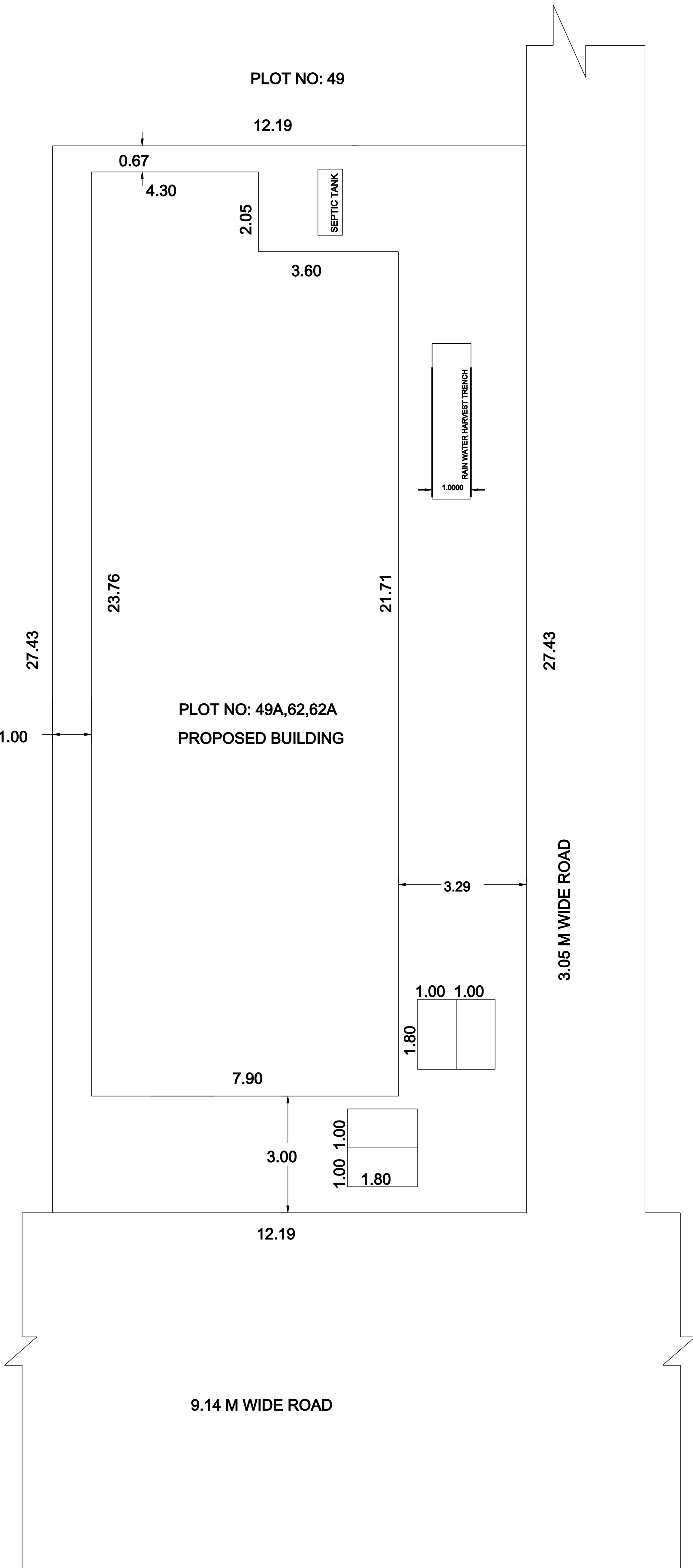
SITE PLAN
