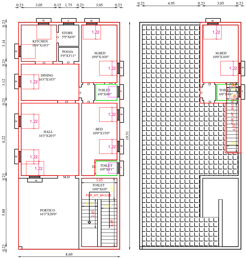
GROUND PLAN
