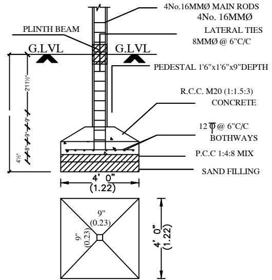
FOUNDATION DETAIL
