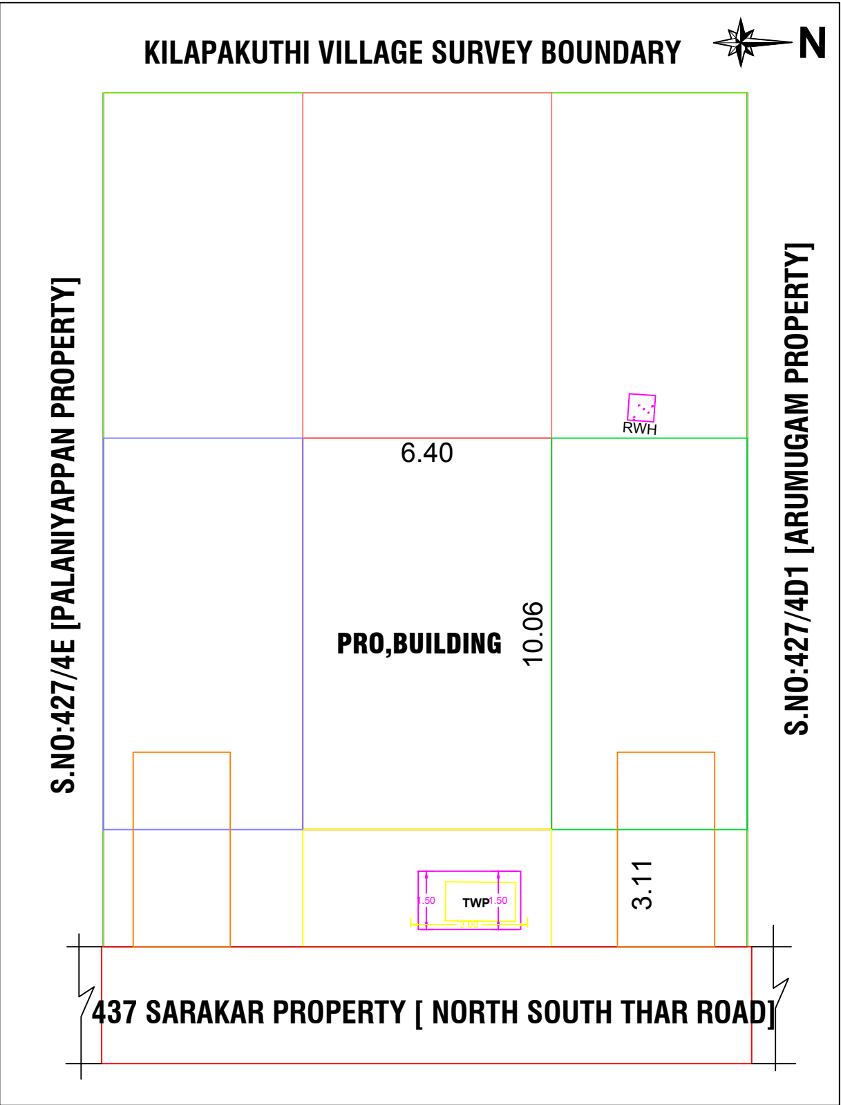
SITE PLAN
