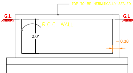
RWH_CAPACITY_L=2000LTRS
