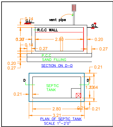
PLAN OF SEPTIC TANK SCALE 1"=2'0"
