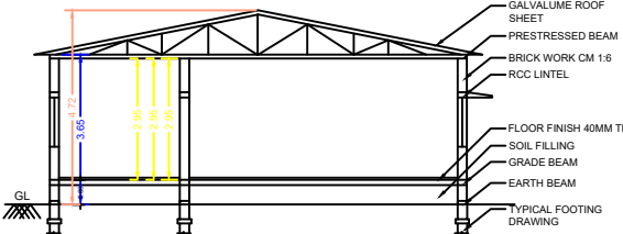
SECTION A - B
