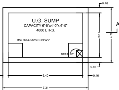
SUMP DETAIL SCALE 1"=4'0"
