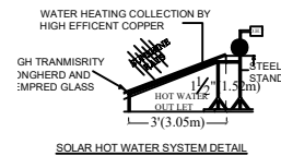
SOLAR HOT WATER SYSTEM DETAIL
