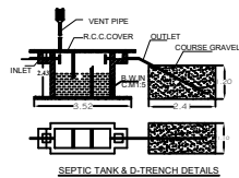
SEPTIC TANK & D-TRENCH DETAILS
