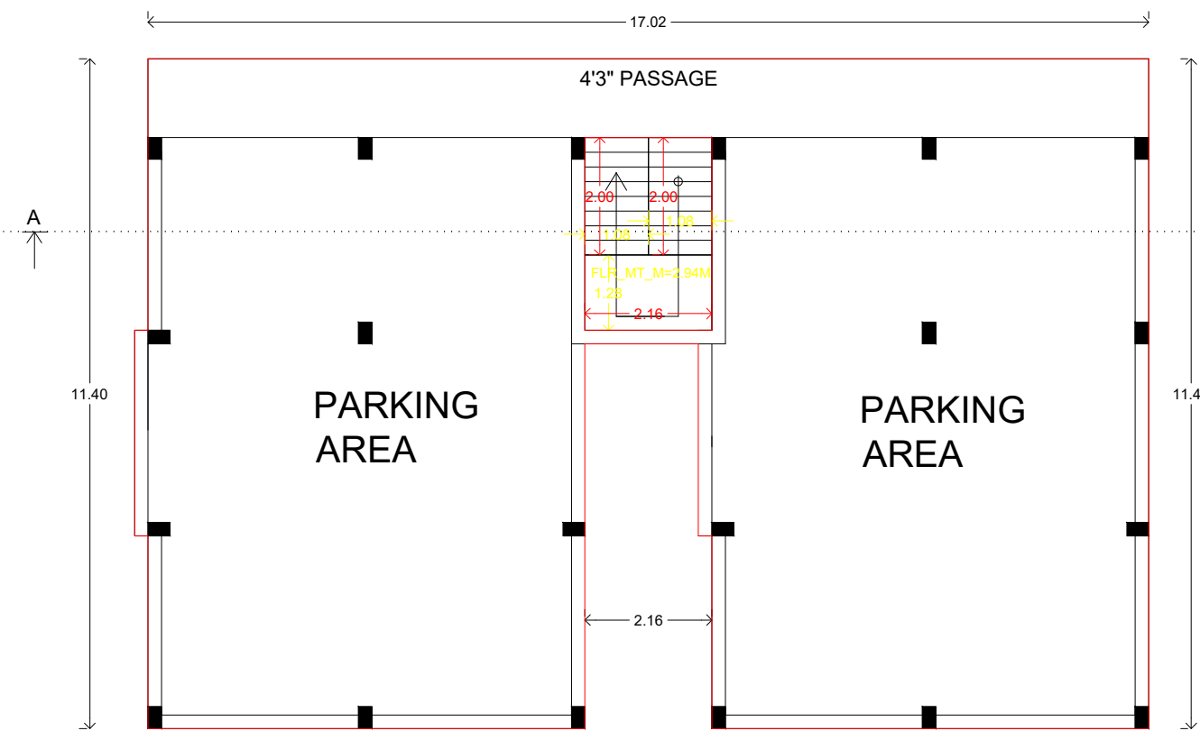
STILT FLOOR PLAN
