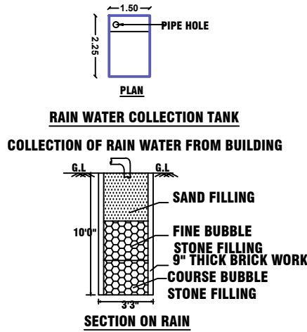
SECTION ON RAIN WATER COLLECTION TANK
