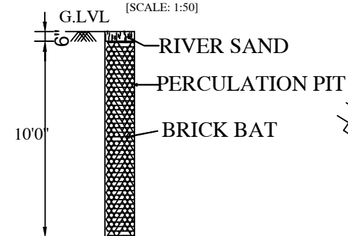
PERCOLATION PIT
