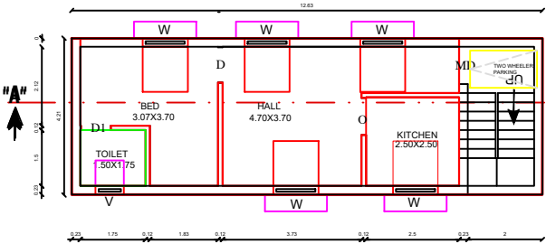
FLOOR - GROUND
