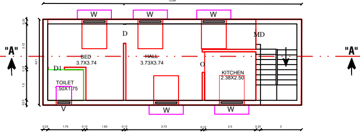
FLOOR - TERRACE PRO.TERRACE FLOOR PLAN
