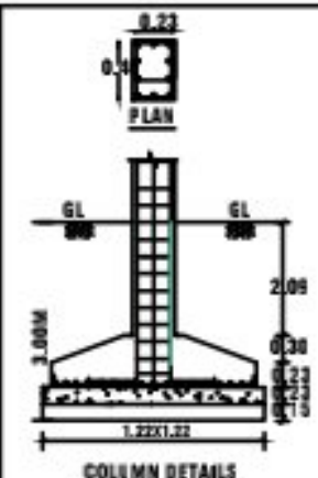
COLUMN DETAILS
