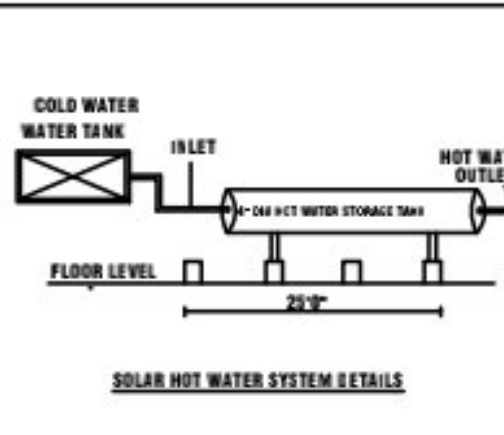
SOLAR HOT WATER SYSTEM DETAILS
