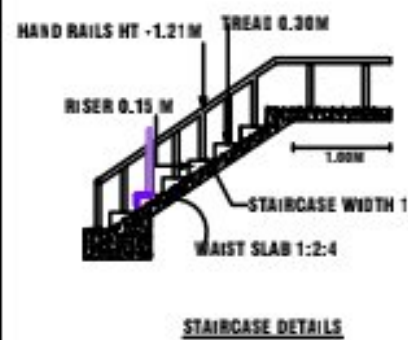
STAIRCASE DETAILS
