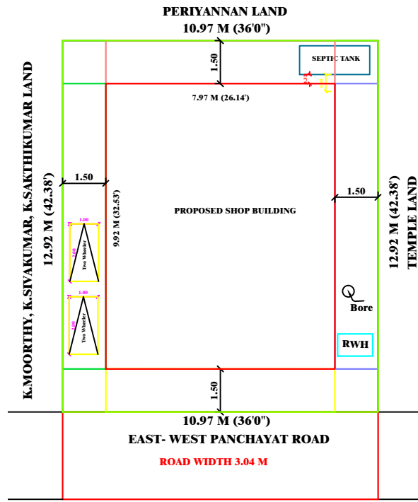
SITE PLAN
