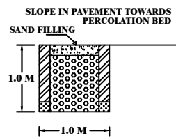
SECTION OF RAIN WATER PERCOLATION BED
