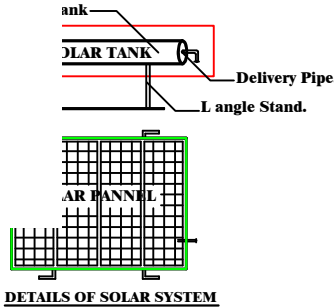
DETAILS OF SOLAR SYSTEM
