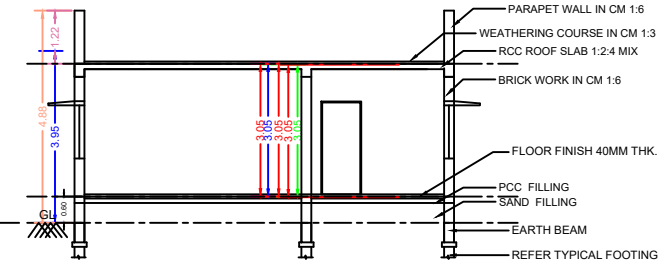
SECTION A - B
