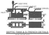
SEPTIC TANK & D-TRENCH DETAILS (NOT TO SCALE)
