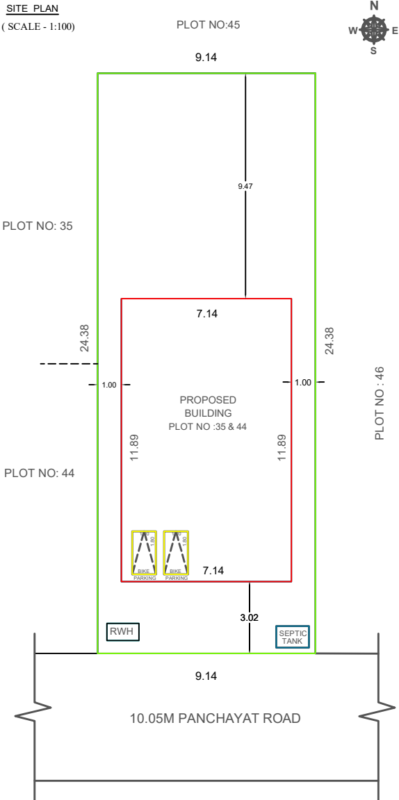
PLAN
