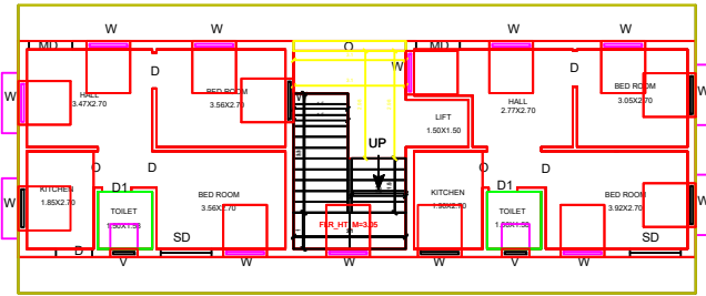
PRO.TYPICAL FLOOR PLAN - FIRST AND SECOND FLOOR
