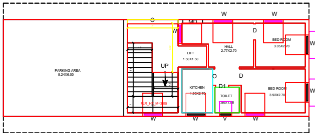
FLOOR - GROUND PRO.GROUND FLOOR PLAN
