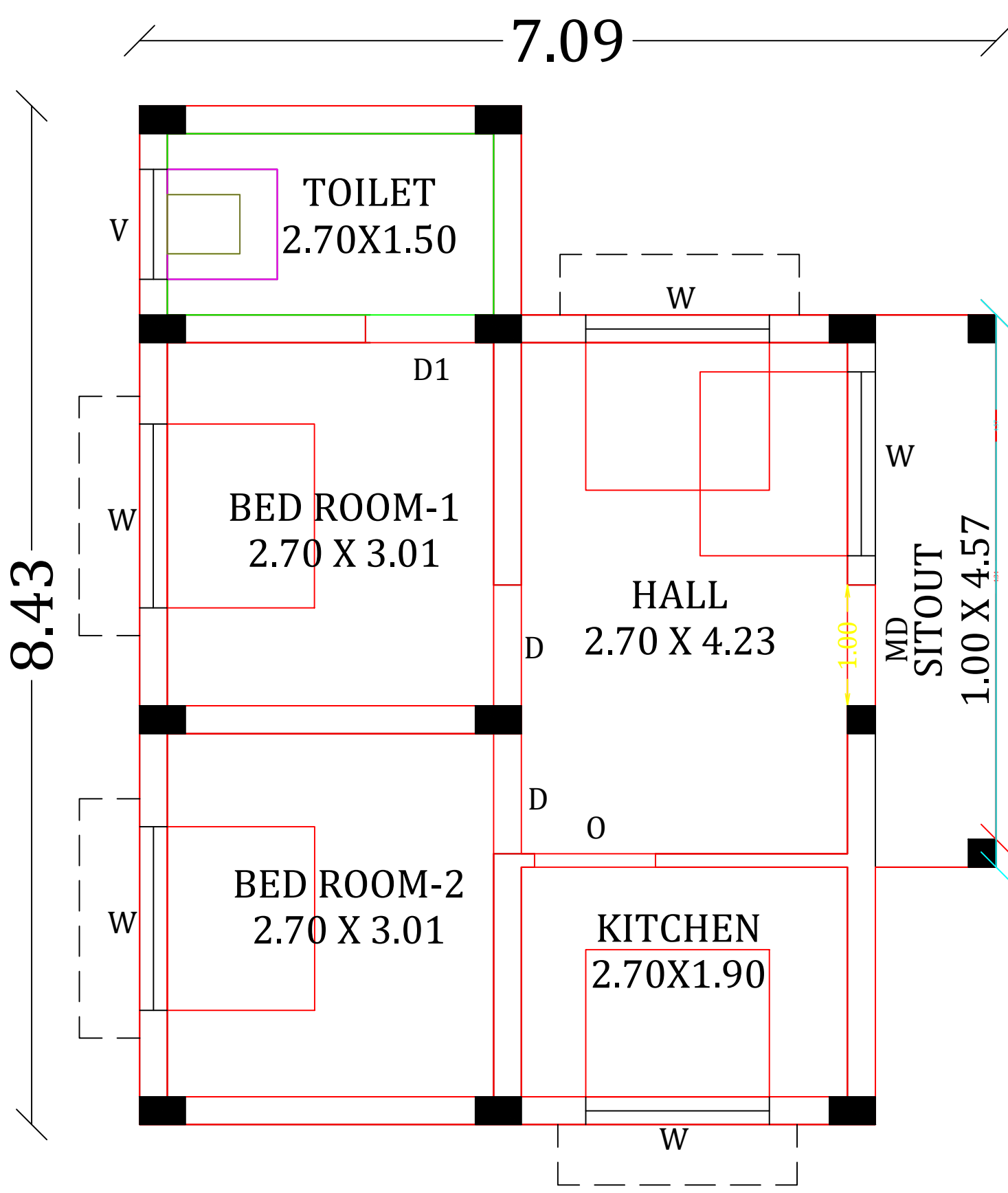
FLOOR-GROUND PRO. GROUND FLOOR PLAN
