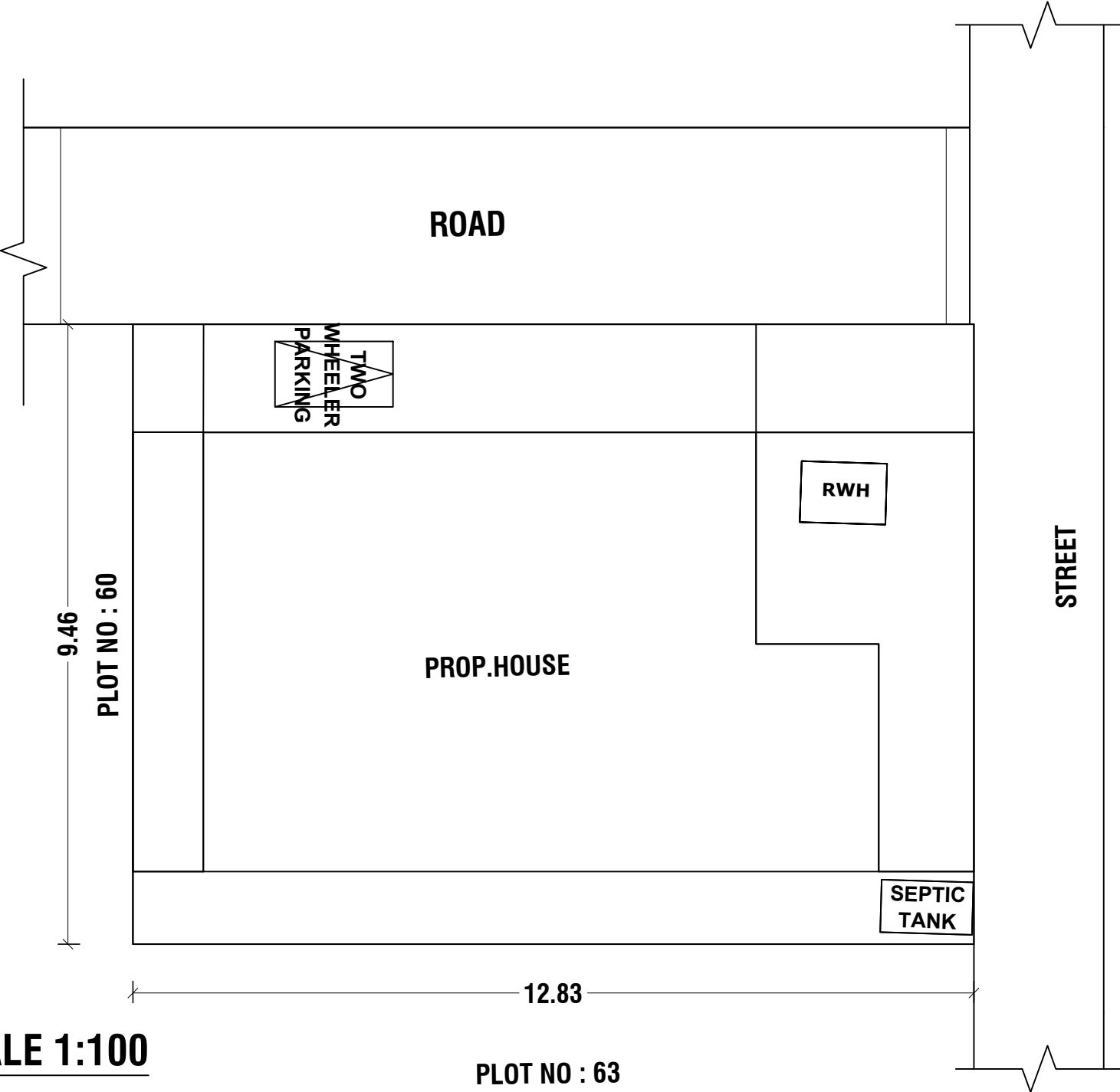
SITE PLAN
