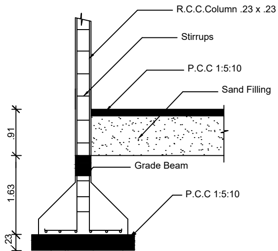
COLUMN DETAIL
