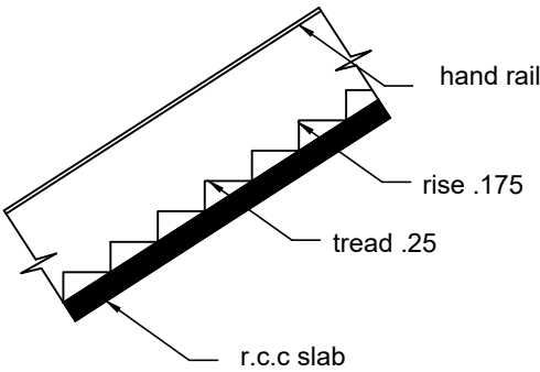
STAIR
