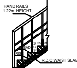
SECTION ON STAIRCASE
