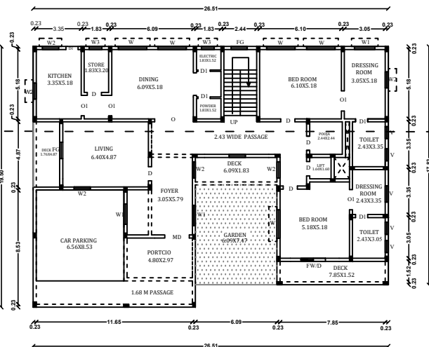
FLOOR- GROUND PRO.GROUND FLOOR PLAN
