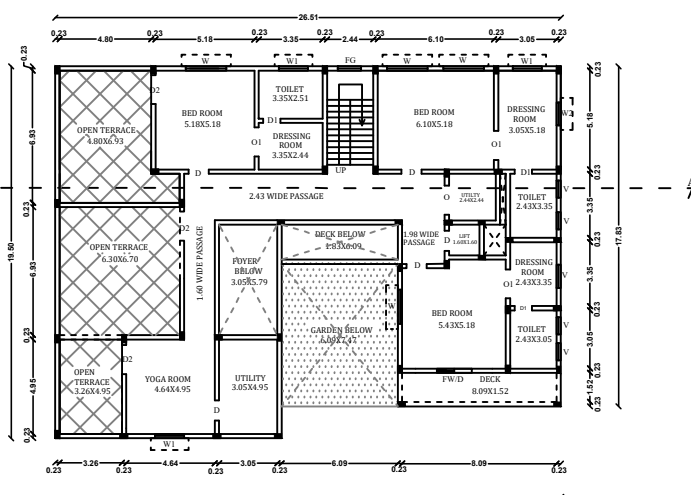
FLOOR- FIRST PRO.FIRST FLOOR PLAN
