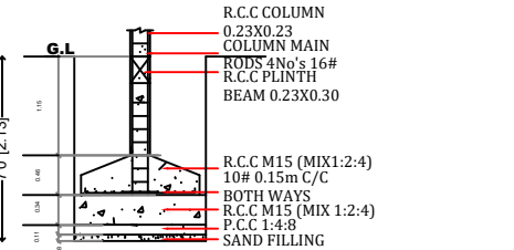
FOUNDATION DETAILS
