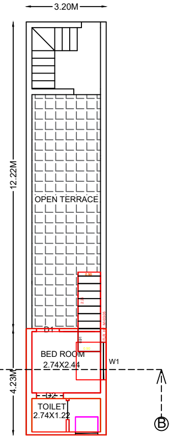
PROPOSED FIRST FLOOR PLAN
