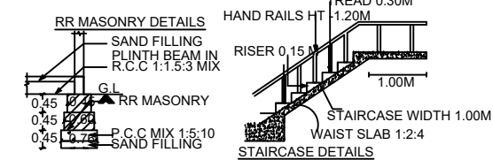
RR MASONRY DETAILS
