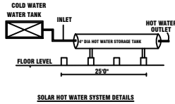
SOLAR HOT WATER SYSTEM DETAILS
