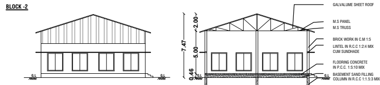
SOUTH SIDE ELEVATION
