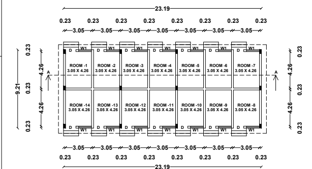
BLOCK -4 PRO.GROUND FLOOR PLAN
