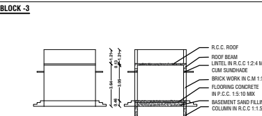
SOUTH SIDE ELEVATION
