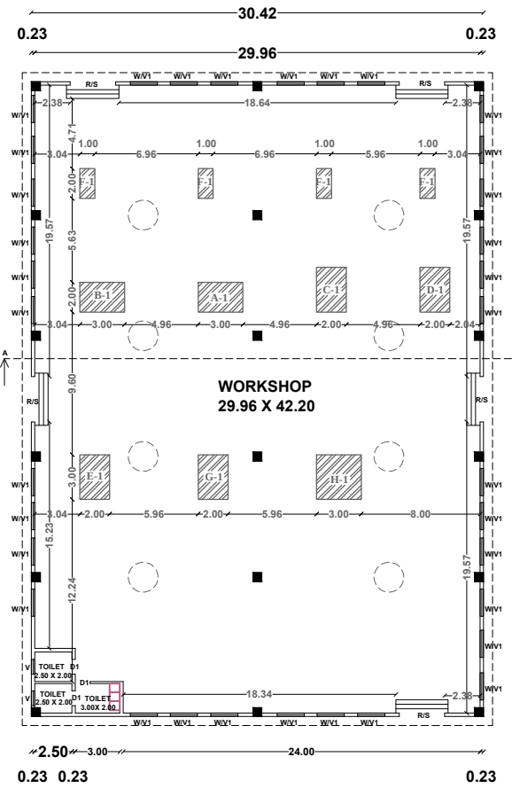
BLOCK -1 PRO.GROUND FLOOR PLAN
