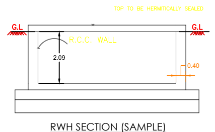
RWHP_CAPACITY_L=2000LTRS
