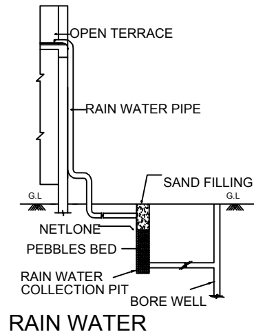
RAIN WATER
