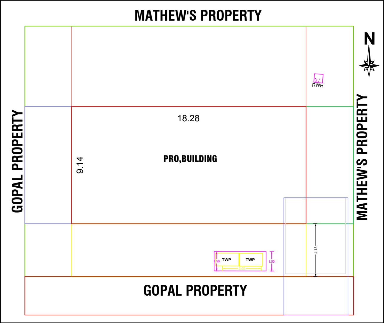
SITE PLAN
