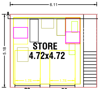
PRO.,GROUND FLOOR PLAN
