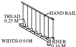
STAIRCASE DETAILS
