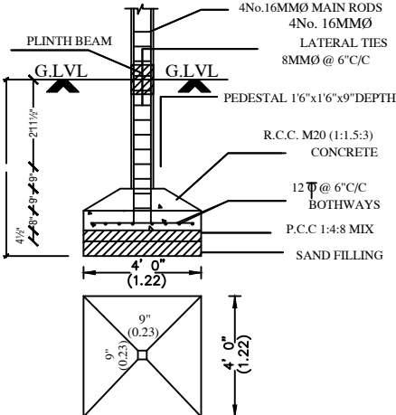
FOUNDATION DETAIL
