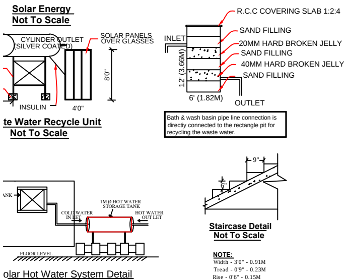
olar Hot Water System Detail
