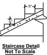
Staircase Detail Not To Scale
