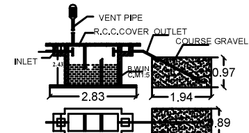
SEPTIC TANK & D-TRENCH DETAILS NOT TO SCALE
