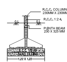
FOUNDATION DETAIL (NOT TO SCALE)
