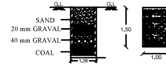
SECTION NO RAIN WATER COLL. TANK
