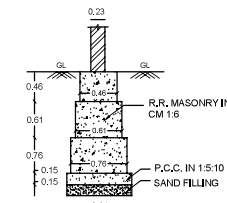
FOOTING DETAIL (NOT TO SCALE)
