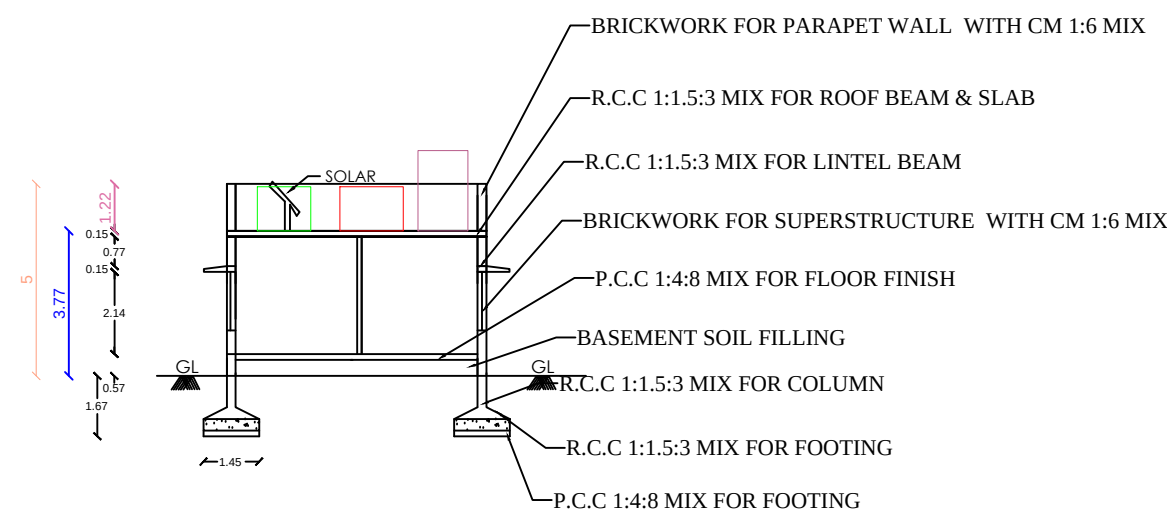
SECTION ON A.
