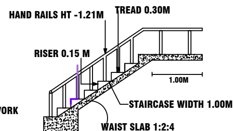
STAIRCASE DETAIL
