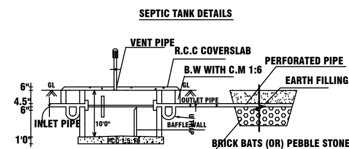
SECTION OF S.P.T & I
