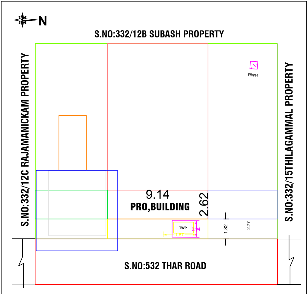
SITE PLAN
